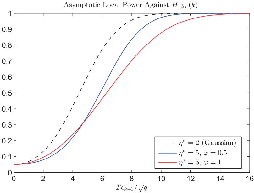
Figure 4. Asymptotic local power of statistic S(k) under local alternatives in a non-Gaussian setting: we take T=2 , k=0 , nominal size \alpha = 0.05 , and \eta^* = \eta/q = 5 . The parameter \varphi = Q_{11}^2 is the squared upper-left element of matrix Q .
