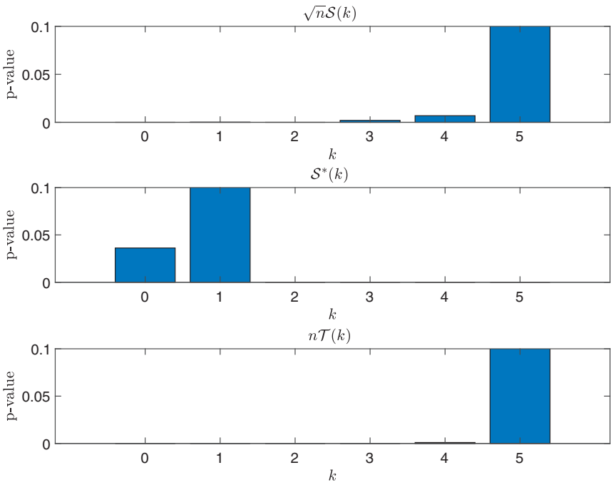
Figure 10. The figure displays the p-values for statistics S(k) (upper panel), S^*(k) (middle panel), and T(k) (lower panel) for the period from December 2010 to November 2011. This period is classified as “bull market” according to Lunde and Timmermann (2004) methodology.
