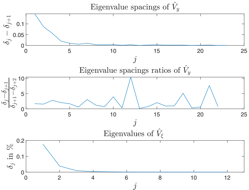
Figure 11. Eigenvalue spacings of matrix \hat{V}_y (upper panel), their ratios (middle panel), and eigenvalues of matrix \hat{V}_\xi (lower panel) for the period from January 2020 to December 2021. We associate this period in our sample to the Covid-19 pandemic.
