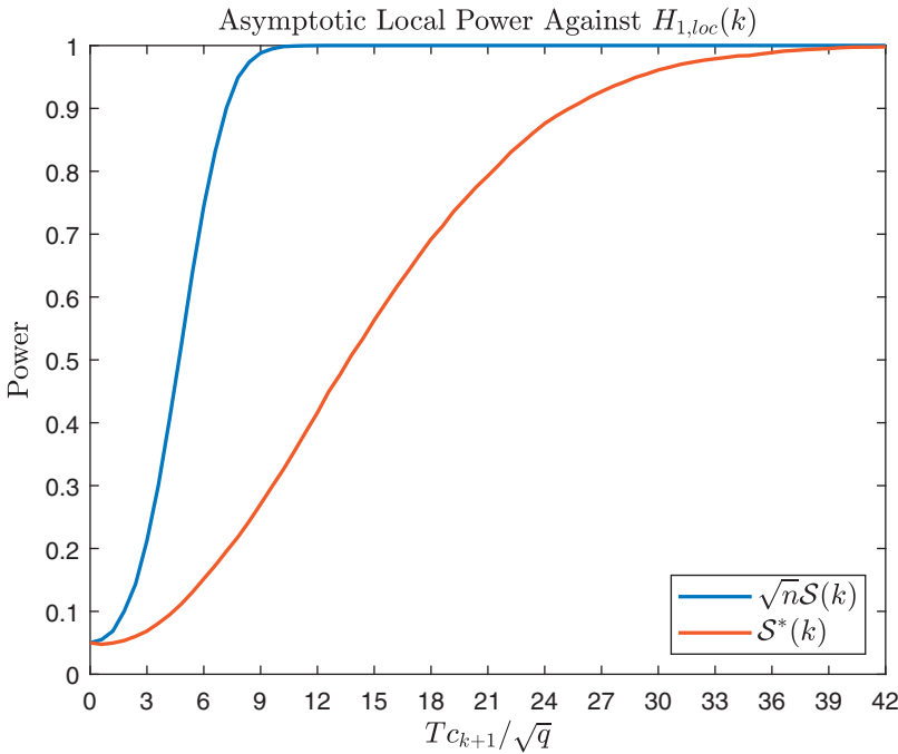
Figure 3. Asymptotic local power under local alternatives in a Gaussian setting: we take T - k = 3 , and nominal size \alpha = 0.05 . We use 10,000 draws of the symmetric matrix Z = (z_{ij}) with z_{ii} \sim N(0, 2q) and z_{ij} \sim N(0, q) for i \neq j .
