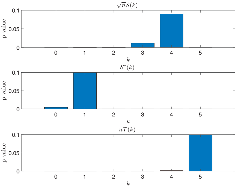
Figure 6. The figure displays the p-values for statistics S(k) (upper panel), S^*(k) (middle panel), and T(k) (lower panel) for the period from March 1977 to February 1978. This period is classified as “bull market” according to Lunde and Timmermann (2004) methodology.
