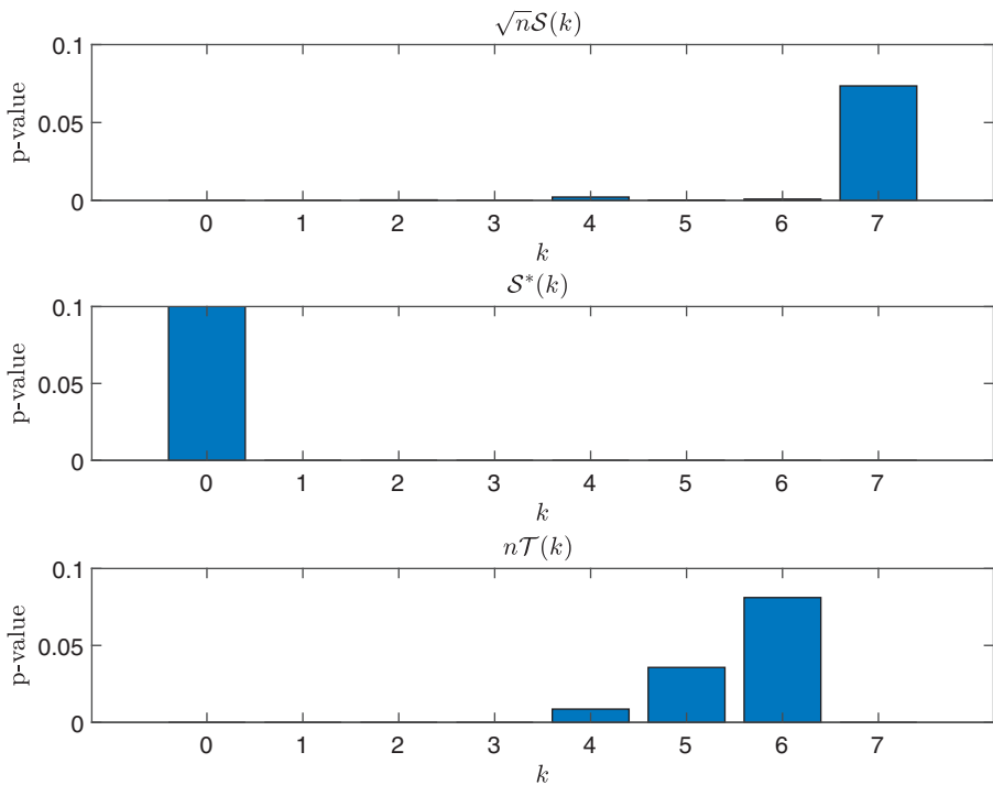
Figure 12. The figure displays the p-values for statistics \mathcal{S}(k) (upper panel), \mathcal{S}^*(k) (middle panel), and \mathcal{T}(k) (lower panel) for the period from January 2020 to December 2021. We associate this period in our sample to the Covid-19 pandemic.
