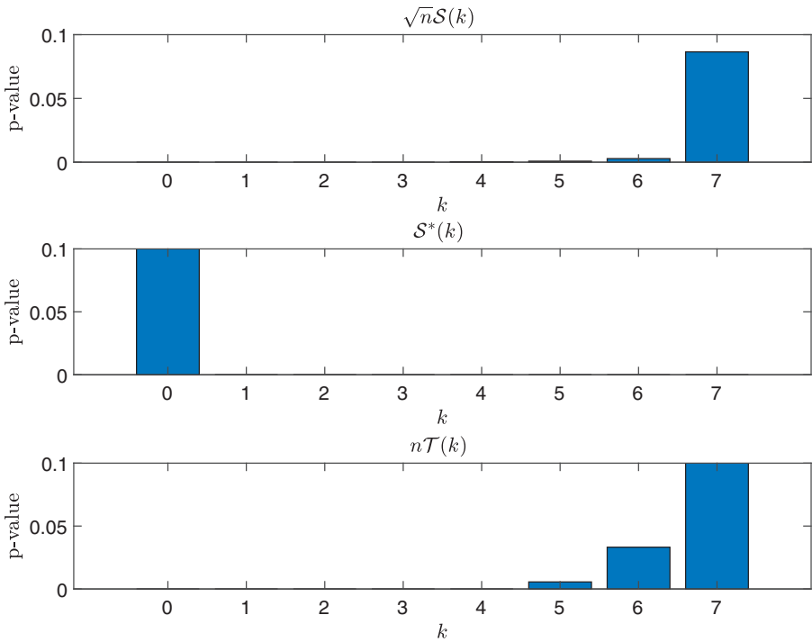
Figure 8. The figure displays the p-values for statistics \mathcal{S}(k) (upper panel), \mathcal{S}^*(k) (middle panel), and \mathcal{T}(k) (lower panel) for the period from July 1981 to June 1982. This period is classified as “bear market” according to Lunde and Timmermann (2004) methodology.
