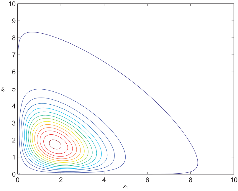
Figure 1. Level curves for the joint pdf of eigenvalue spacings s_1 = \delta_1(Z^*) - \delta_2(Z^*) and s_2 = \delta_2(Z^*) - \delta_3(Z^*) for random matrix Z^* in \text{GOE}(3) .
