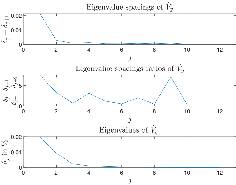
Figure 7. Eigenvalue spacings of matrix \hat{V}_y (upper panel), their ratios (middle panel), and eigenvalues of matrix \hat{V}_\xi (lower panel) for the period from July 1981 to June 1982. This period is classified as “bear market” according to Lunde and Timmermann (2004) methodology.
